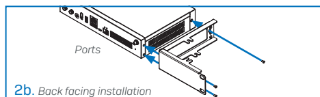
2b. Back facing installation
