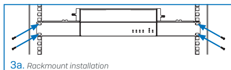
3a. Rackmount installation
