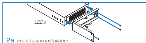
2a. Front facing installation
